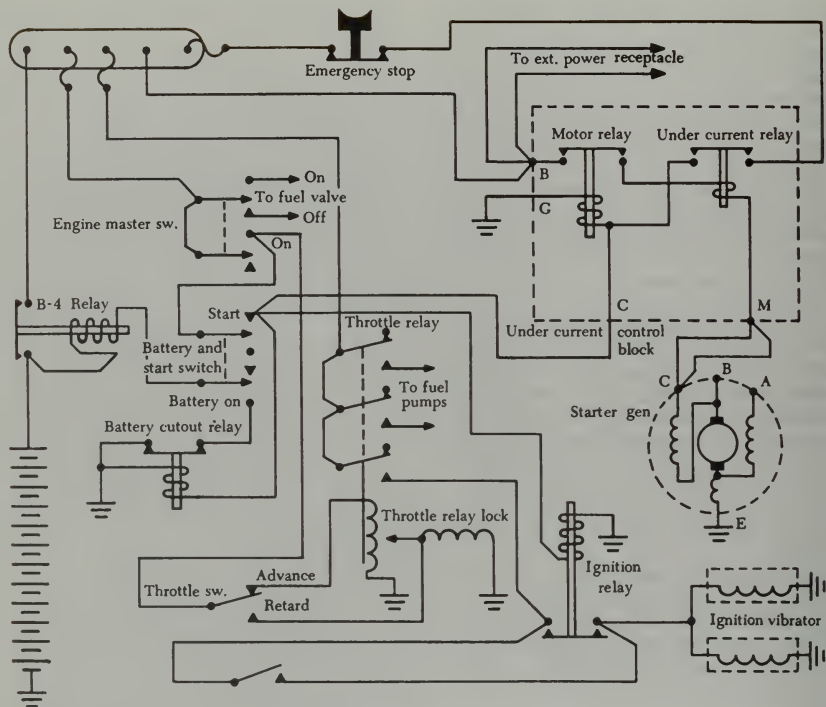
FIGURE 5-15. Starter-generator circuit.
